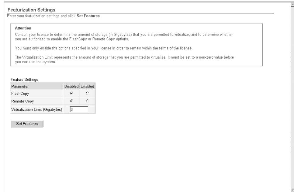
Figure 44. Featurization settings
