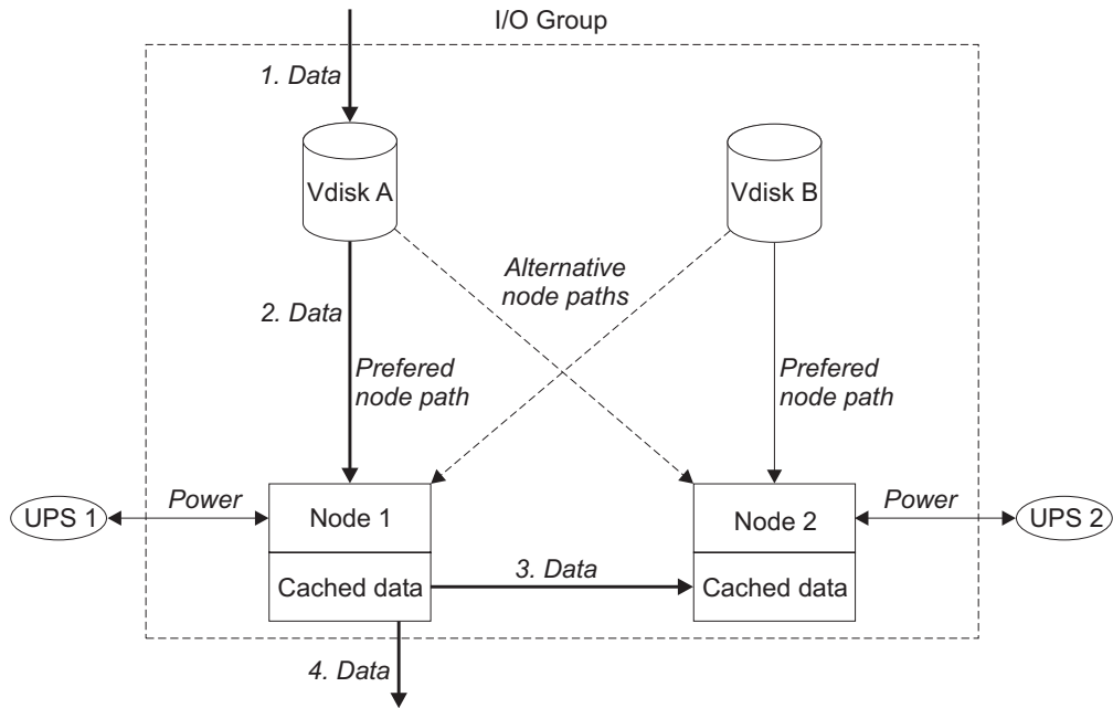
Figure 9. I/O group and uninterruptible power supply
