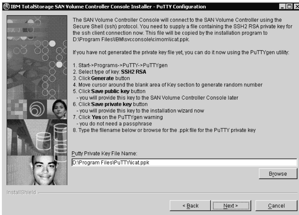
Figure 50. PuTTY Configuration panel
