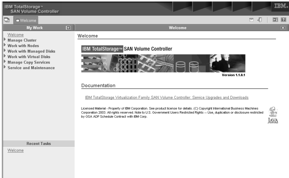
Figure 35. Welcome panel
