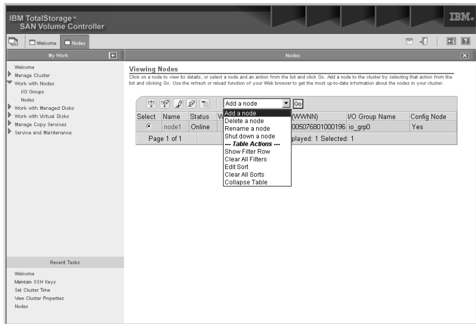
Figure 40. Add node drop down list
