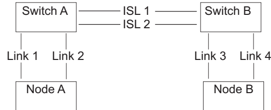
Figure 20. Fabric with Inter-Switch Links between nodes in a cluster
