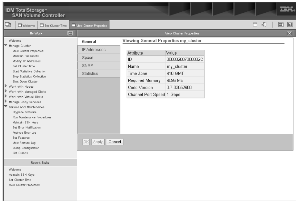
Figure 37. View Cluster properties panel
