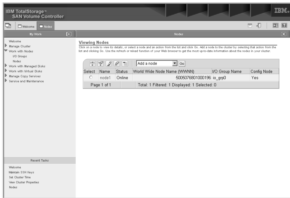
Figure 39. Nodes panel
