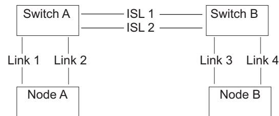
Figure 8. Fabric with ISL between nodes in a cluster
